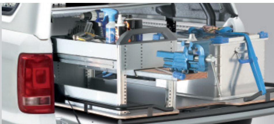
Bench module with retractable vice and sectioned storage compartment Art. W502104
